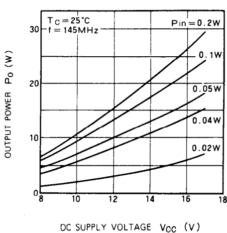
OUTPUT POWER VS. DC SUPPLY VOLTAGE
